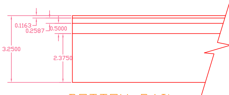
BOTTOM RAIL TOP VIEW
