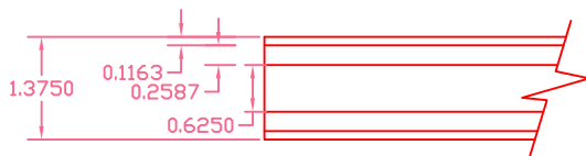
BOTTOM RAIL FRONT VIEW
