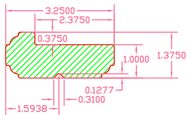
BOTTOM RAIL END VIEW
