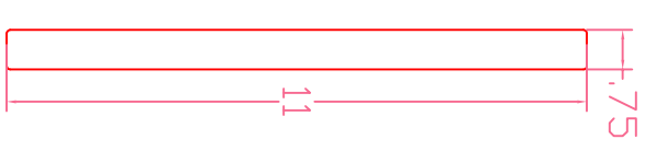
FASCIA END VIEW
