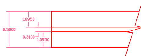
TOP RAIL BASE TOP VIEW
