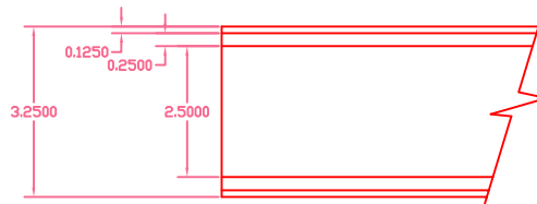
TOP RAIL CAP TOP VIEW
