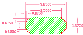
TOP RAIL CAP END VIEW
